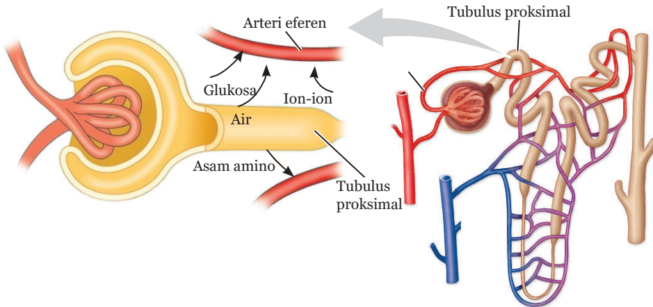
Gambar 9.6 Proses Reabsorpsi
